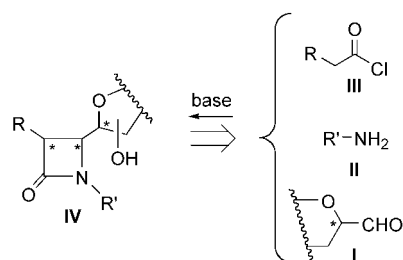
Figure 1. Reagents I – III for a multicomponent synthesis of C -glycosyl-β-lactams IV .
