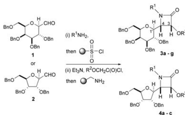
Scheme 1. Reagents and conditions: (i) R 1 NH 2 (1.5 equivs.), 4 Å MS, CH 2 Cl 2 , 0 °C, 1 h, then polymer-bound sulfonyl chloride, 0 °C, 45 min; (ii) Et 3 N (6.0 equivs.), (α-oxy)acetyl chloride (3.5 equivs.), CH 2 Cl 2 , –50 °C to r.t., 12 h, then aminomethylated polystyrene, r.t., 4 h.
