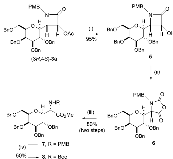
Scheme 2. Reagents and conditions: (i) LiOH (2.0 equivs.), 30% H 2 O 2 (6.0 equivs.), THF-H 2 O (3:1), 0 °C, 2 h; (ii) TEMPO (1.0 equiv.), NaOCl, KBr, buffer phosphate solution, CH 2 Cl 2 , 0 °C, 15 min; (iii) MeOH, 50 °C, 8 h; (iv) Boc 2 O (2.0 equivs.), dioxane, r.t., 24 h; then CAN (3.0 equivs.), MeCN-H 2 O (4:1), r.t., 2 h.
