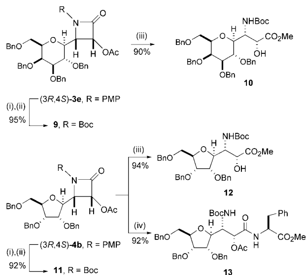
Scheme 3. Reagents and conditions: (i) CAN (4.5 equivs.), MeCN-H 2 O (4:1), -10 °C, 2 h; (ii) Boc 2 O (1.5 equivs.), Et 3 N (3.0 equivs.), DMAP (cat.), CH 2 Cl 2 , r.t., 12 h; (iii) Et 3 N (5.0 equivs.), DMAP (3.0 equivs.), MeOH, r.t., 48 h; (iv) H-Phe-OMe.HCl (2.0 equivs.), Et 3 N (4.5 equivs.), DMAP (0.5 equivs.), CH 2 Cl 2 , r.t., 48 h.
